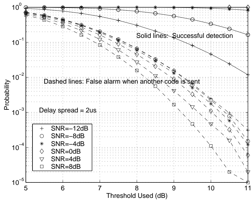
Figure 7. Detection and false alarm rate in the DS=2 \mu s environment
