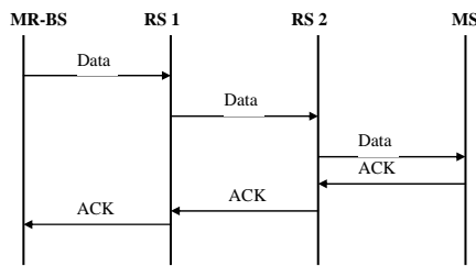
Figure 2. Message Flow for 3-hop DL HARQ
