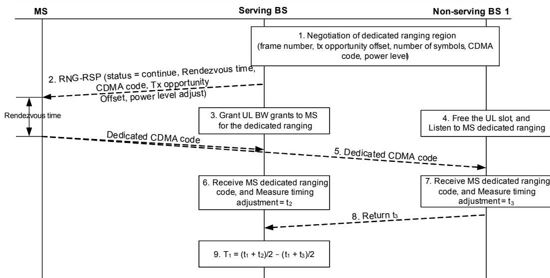
Figure G5 – U-TDOA Measurement Algorithm
